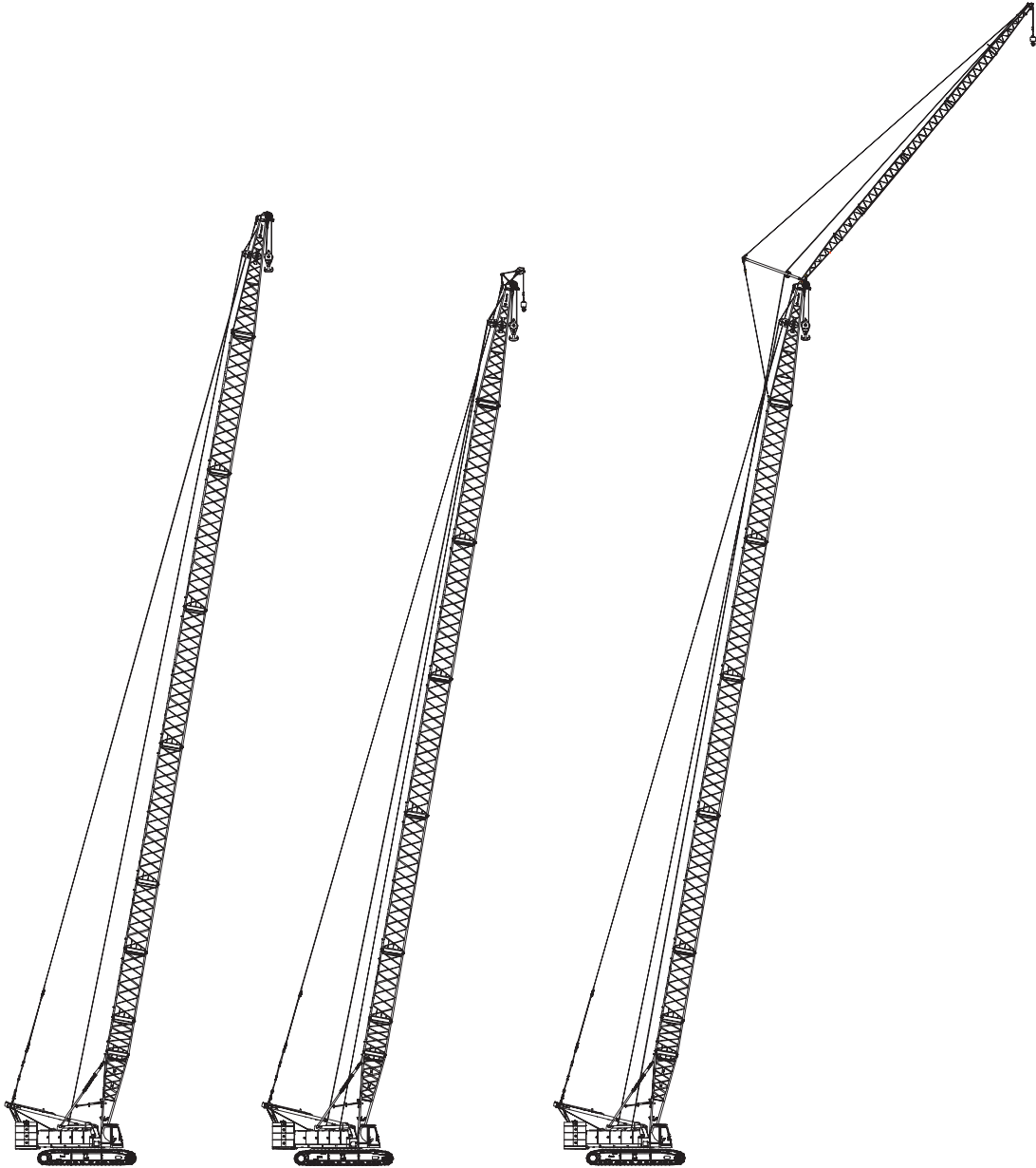
Operating condition of Main boom H (18~81)m (53+16)t
